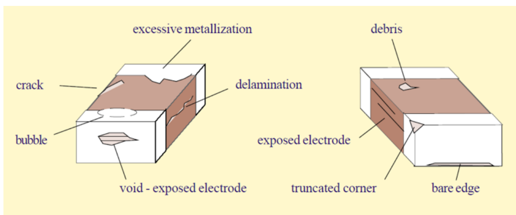
Figure 28. Visual Defects
