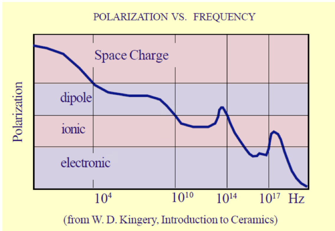
Figure 9: The Effect of Frequency on Polarization Mechanisms
