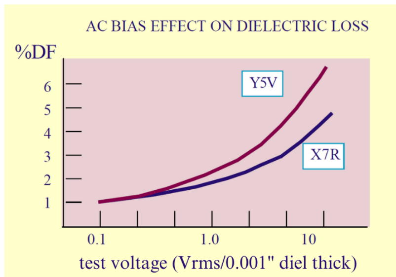
Figure 25. AC Bias Effect on Dielectric Loss
