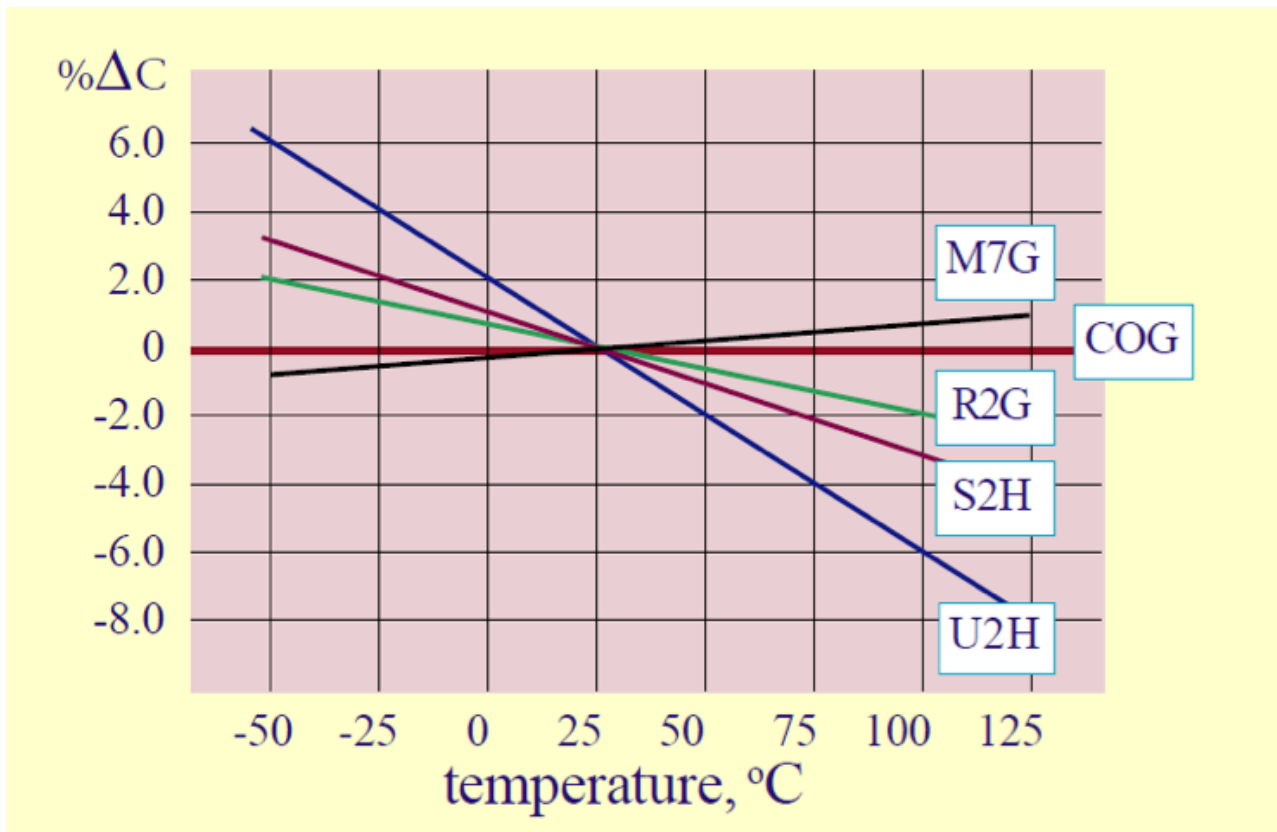
Figure 20. Temperature Coefficients of Linear Dielectrics
