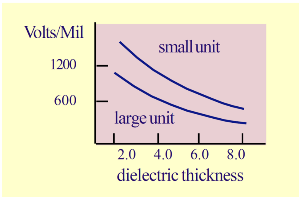
Figure 12: Dielectric Strength vs Dielectric Thickness
